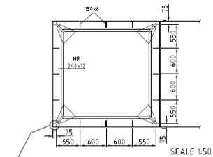
PONTON SECTION FRAMES 5, 7, 9, 13, 15, 17, 21, 23 AND 25 FRAMES 1,5 AND 28,5 EQUIVALENT
